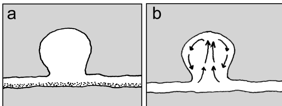
Figure 2: upward growth of anastomoses explained by: a) insoluble residue protecting the lower bed; b) natural convection of water
