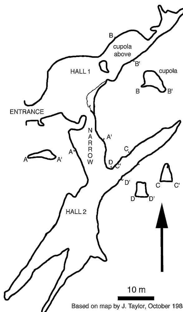
Based on map by J. Taylor, October 1985 Figure 3. Map of Yessabah Bat Cave A Hall & Narrows Cave
