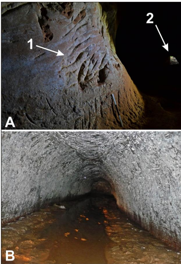
Fig. 12: Two aspects of the surfaces of tunnels of Cenozoic fossorial vertebrates. (A) In the “Toca do Tatu” cave, a concave portion of a smooth lateral wall of the South Tunnel, almost at the intersection with the Hall, shows several preserved digging scratches (Arrow 1). In the back is the rear exit (Arrow 2). Scale (near the floor) = 30 cm. (B) Paleovertebrate tunnel in the municipality of Bom Retiro do Sul (RS) with completely white walls. Width of the tunnel: ~1.2 m.
